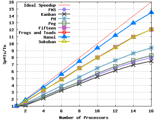
Figure 3. Speedup analysis.
